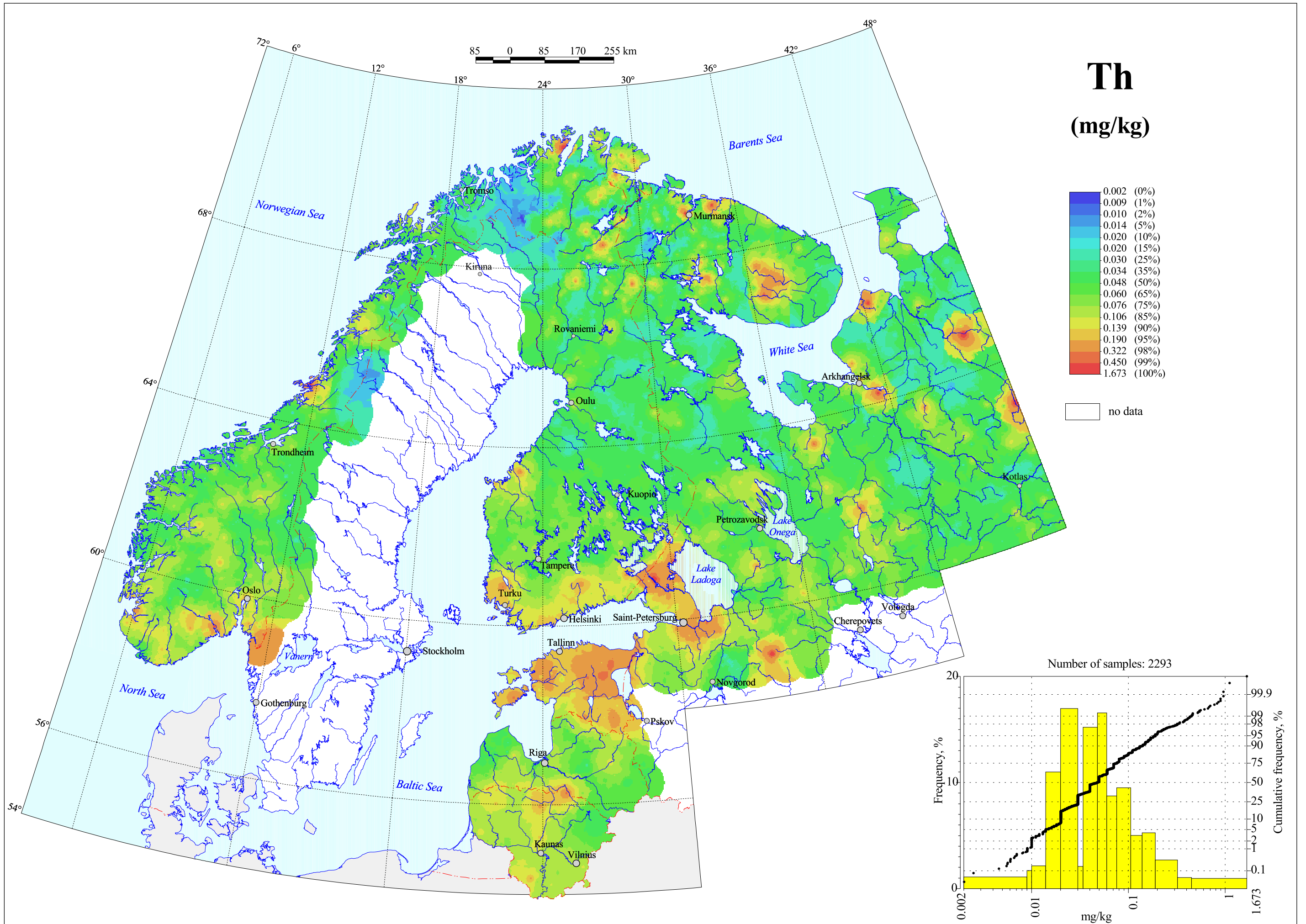
Thorium in Terrestrial Moss, Total Content
